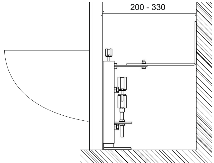
Built-in System with dry wall
