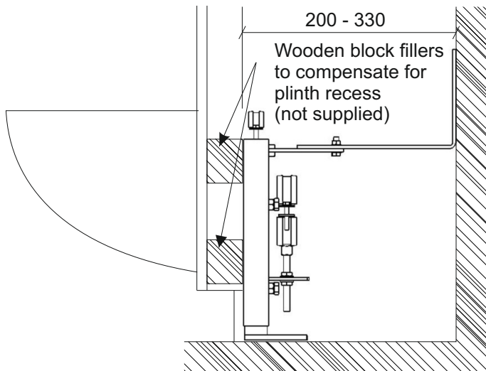
Built-in System in Furniture
